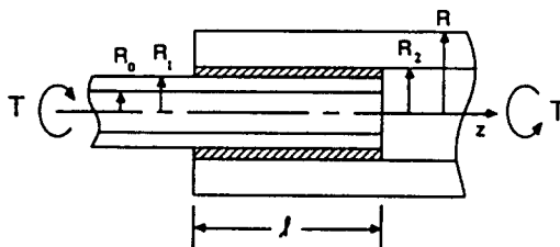
Fig. 1. Adhesive-bonded tubular lap.
