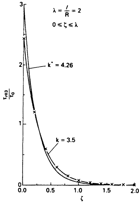
Fig. 5. Distribution of \tau_{\theta 3} for l = 2R .
